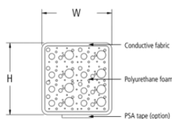
5mm W x 1mm H x 24.5mm L
