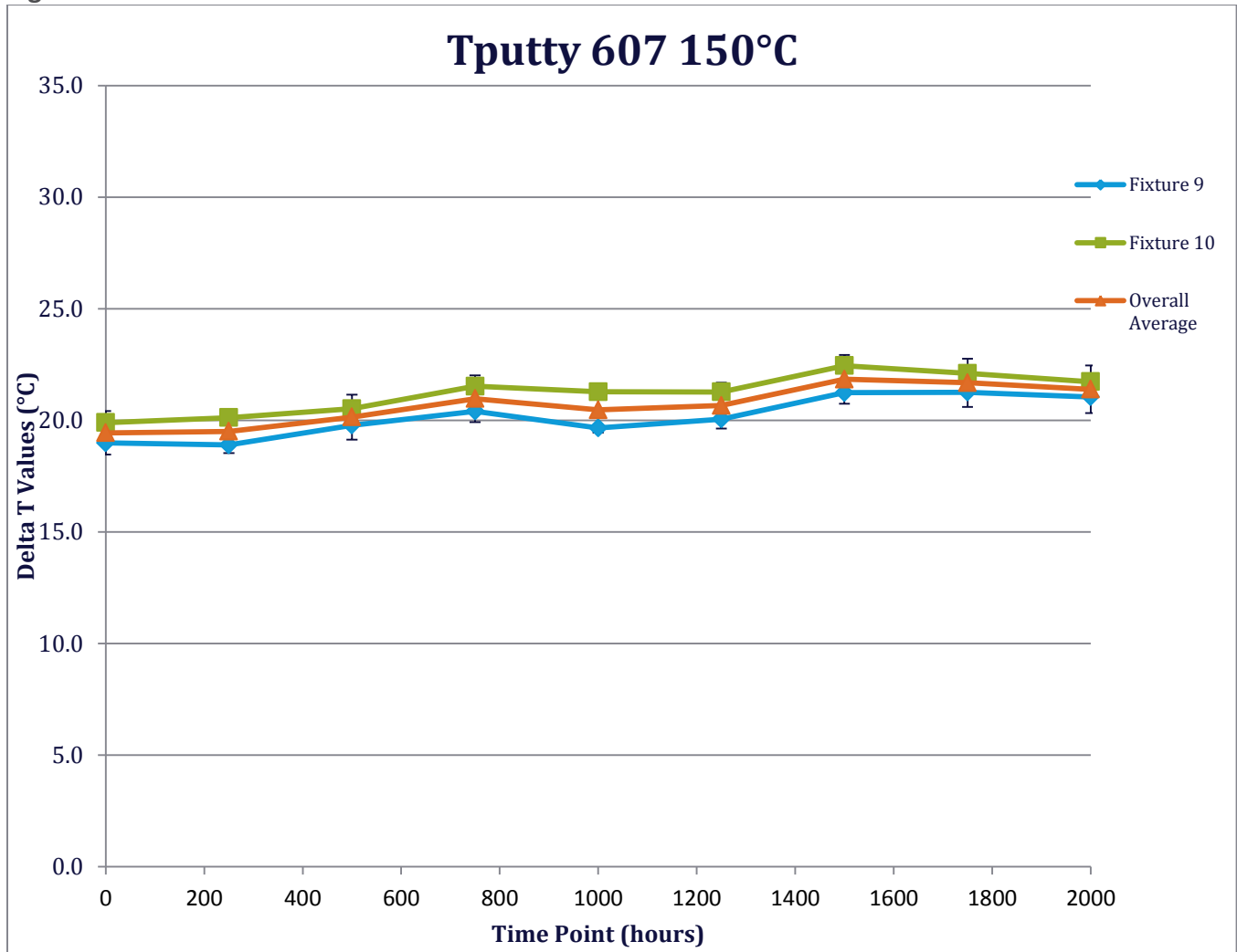
Figure 7: Isothermal Bake Results – 150°C
