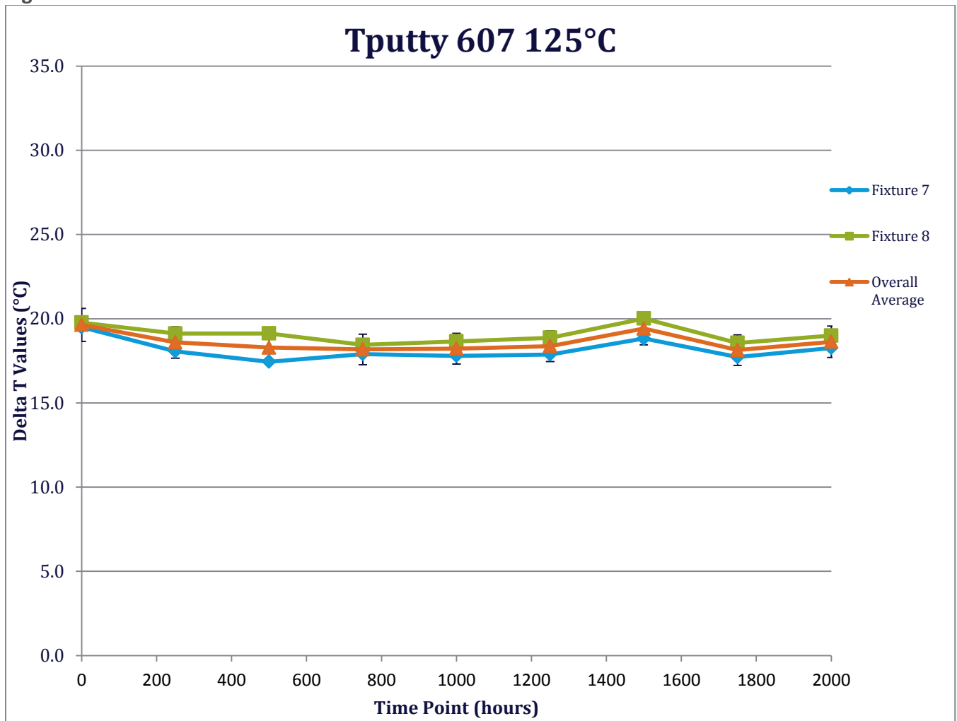
Figure 6: Isothermal Bake Results – 125°C
