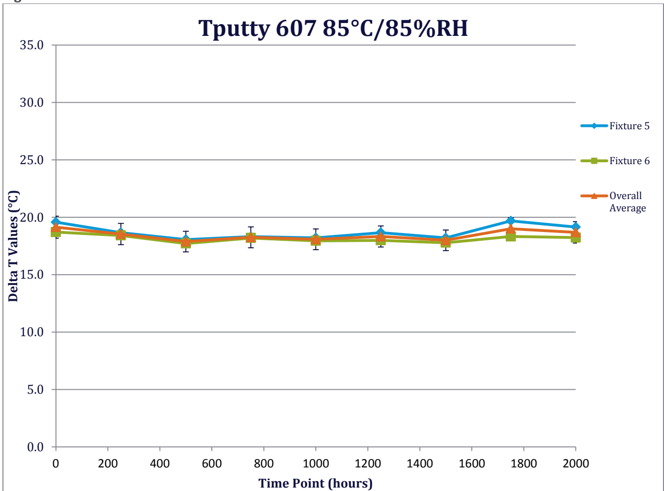
Figure 8: HAST Results
